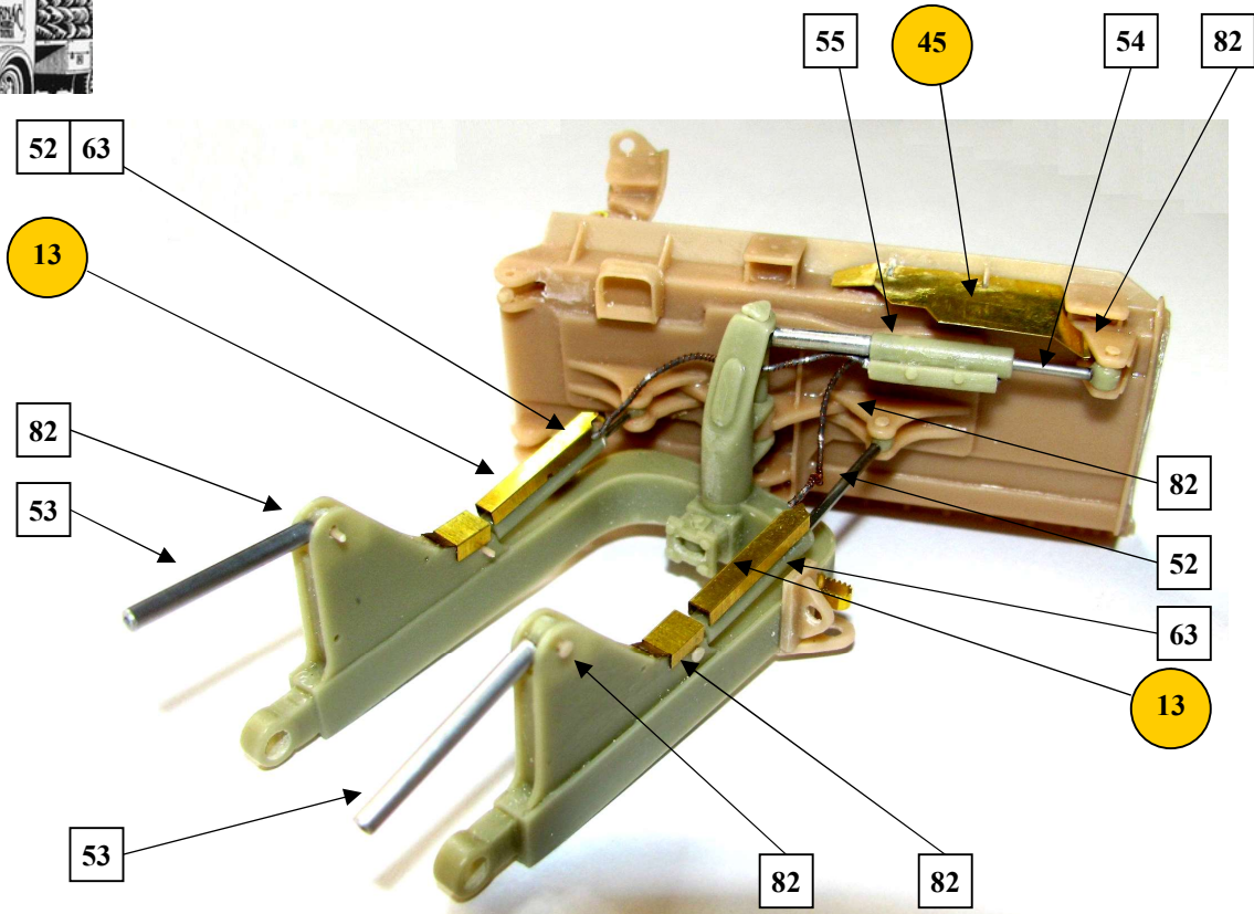
Transport position
