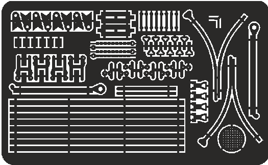
PHOTO-ETCHED PARTS F3065
