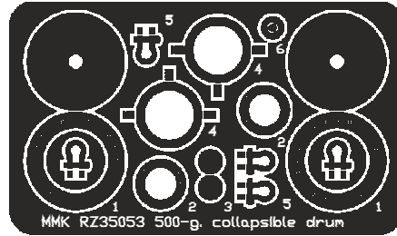
PHOTO-ETCHED PARTS RZ35053
